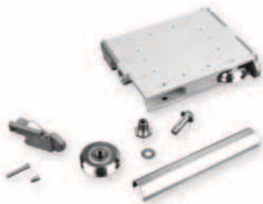
Wiper wheel plate assembly shown consisting of four DualVee wheels, bushings and a carriage plate
